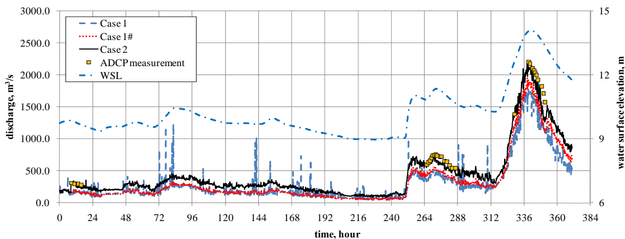
Fig. 10. Time series of water discharges with different methods, water surface elevation, relative errors of Fuji River
