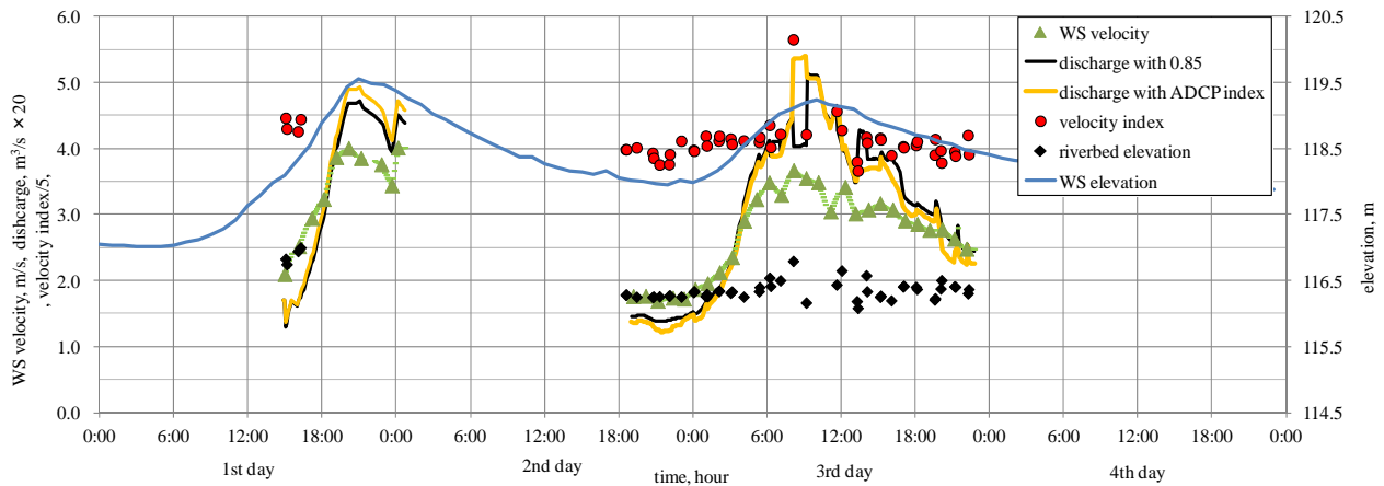
Fig. 7. Time series of river bed elevation, WS elevation, WS velocity, velocity index obtained by ADCP, discharge with velocity index of 0.85 and that by ADCP at section 2
