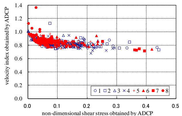
Fig. 6. Relation between non-dimensional shear stress and velocity index by ADCP in Fuji River
