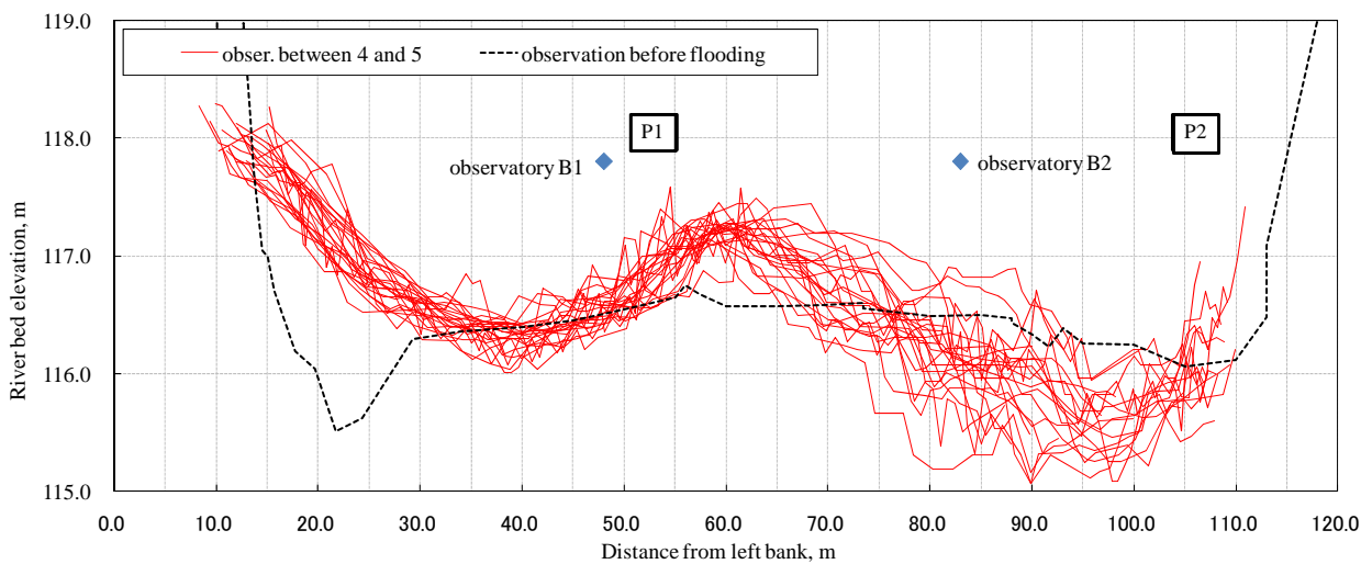
Fig. 3. River bed elevation at different timing using ADCP
