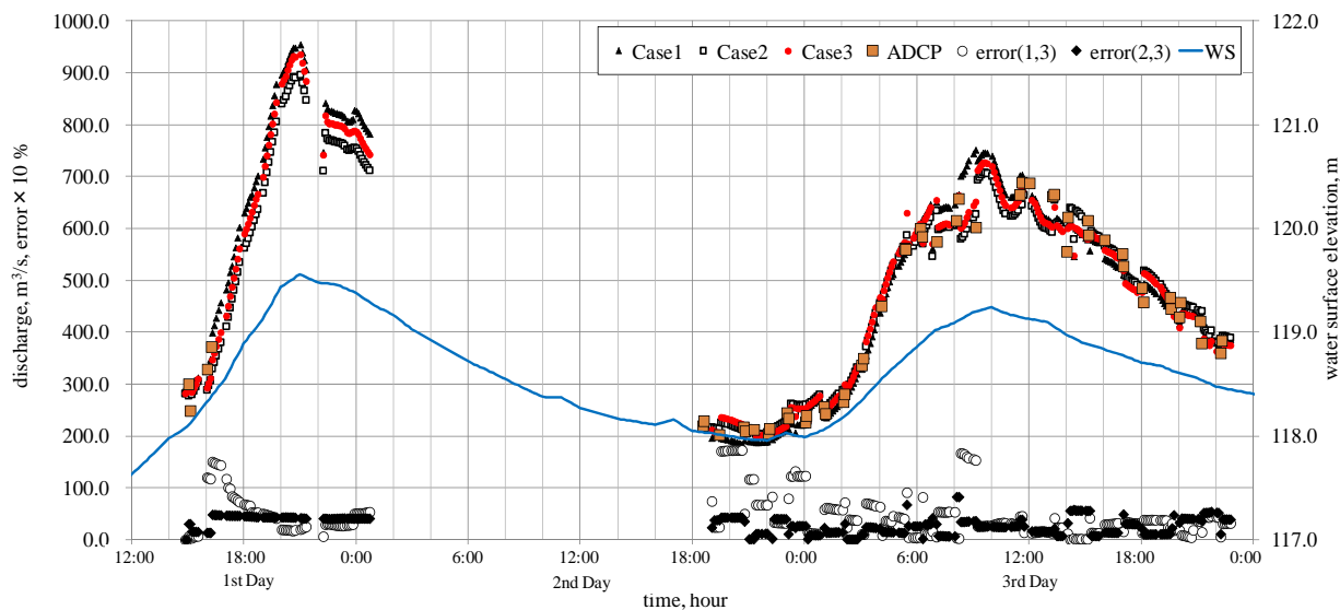
Fig. 9. Time series of water discharges with different methods, water surface elevation, relative errors of Fuji river
