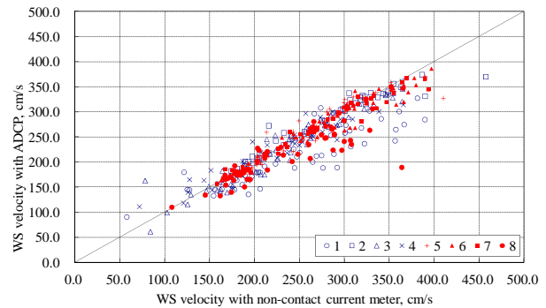
Fig. 4. Comparison of the WS velocity between ADCP and non-contact current meter
