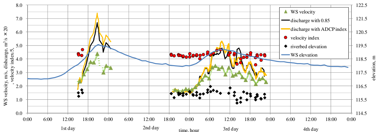
Fig. 8. Time series of river bed elevation, WS elevation, WS velocity, velocity index obtained by ADCP, discharge with velocity index of 0.85 and that by ADCP at section 7
