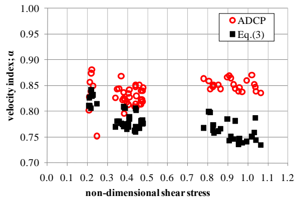
Fig. 5. Relation between non-dimensional shear stress and velocity index by ADCP in Tone River
