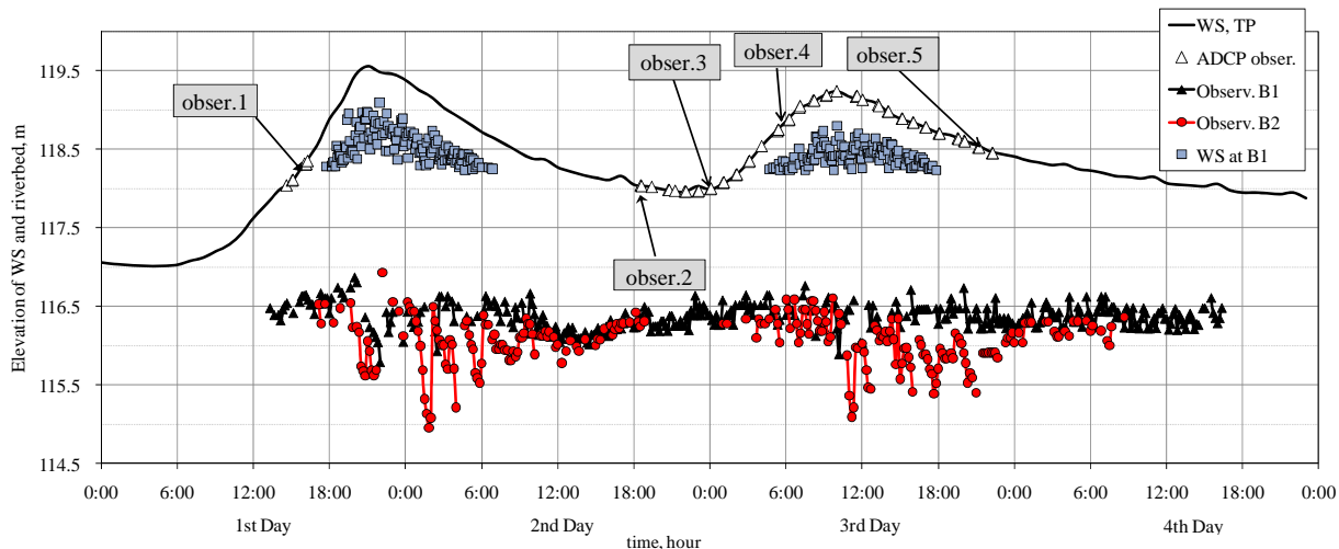
Fig. 2. Time series of river bed elevation, water surface elevation, and timing of ADCP measurements
