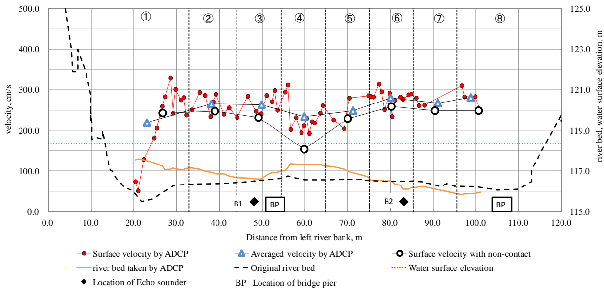
Fig. 1. Cross sectional distribution of velocity and river bed
