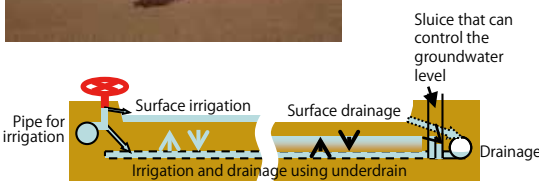
Mechanism of groundwater level control system
