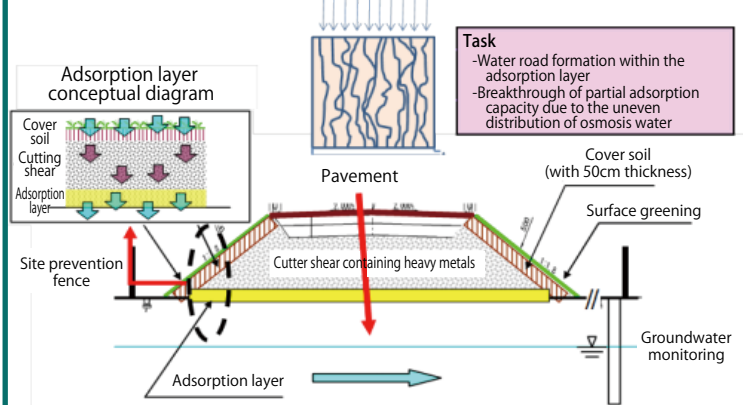
Conceptual diagram of the adsorption layer construction method
