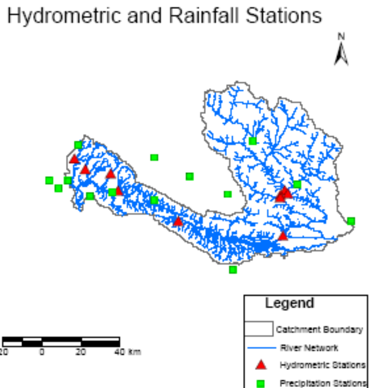
Figure 2.20 West Rapti River Basin with Drainage Network, Rainfall and Hydrometric stations
